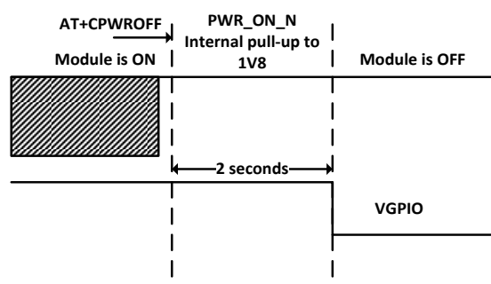
Figure 9. Power OFF Sequence for PWR_ON_N, VGPI0
