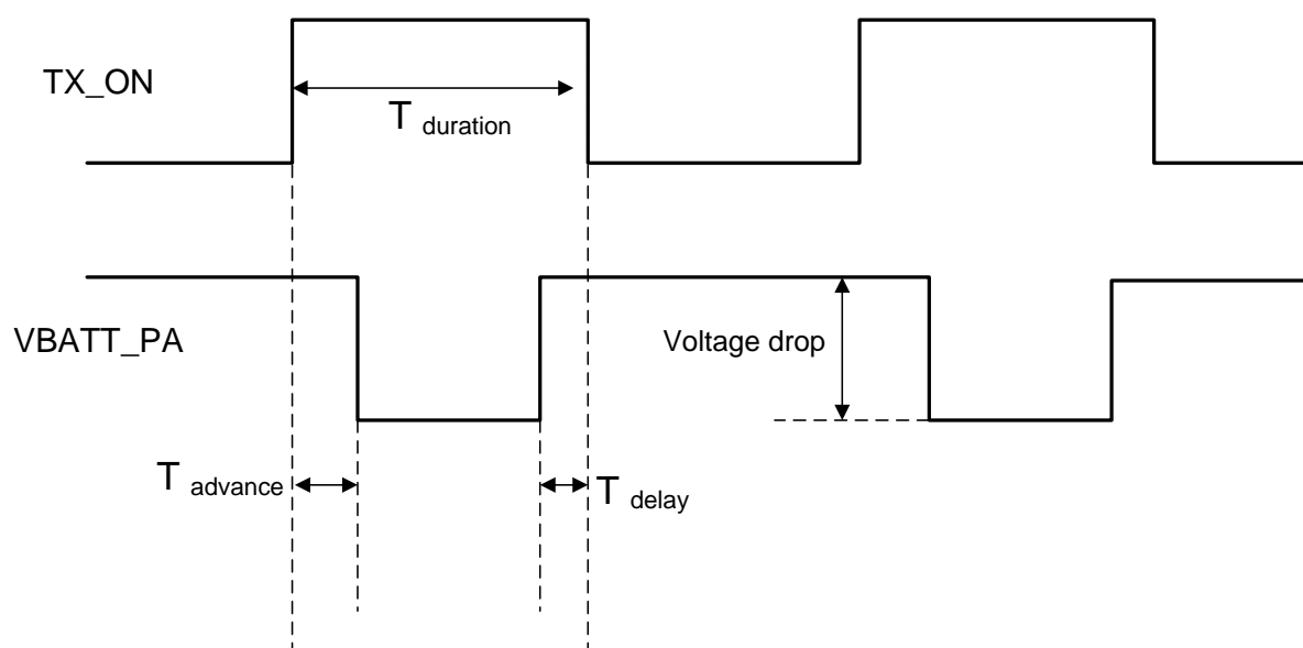
Figure 4. TX_ON State During Transmission
