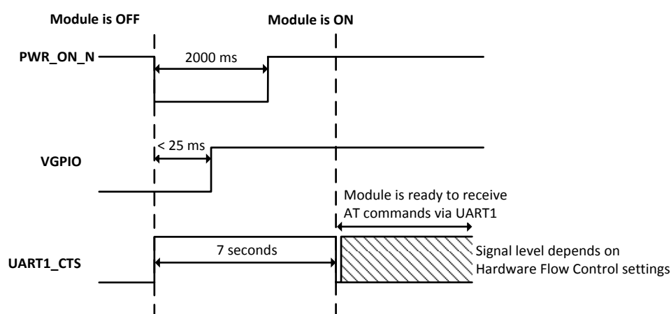
Figure 8. PWR_ON_N Sequence with VGPI0 Information
