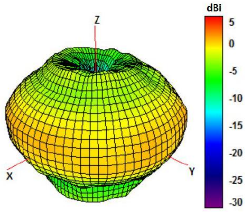
2450 MHz Radiation pattern
